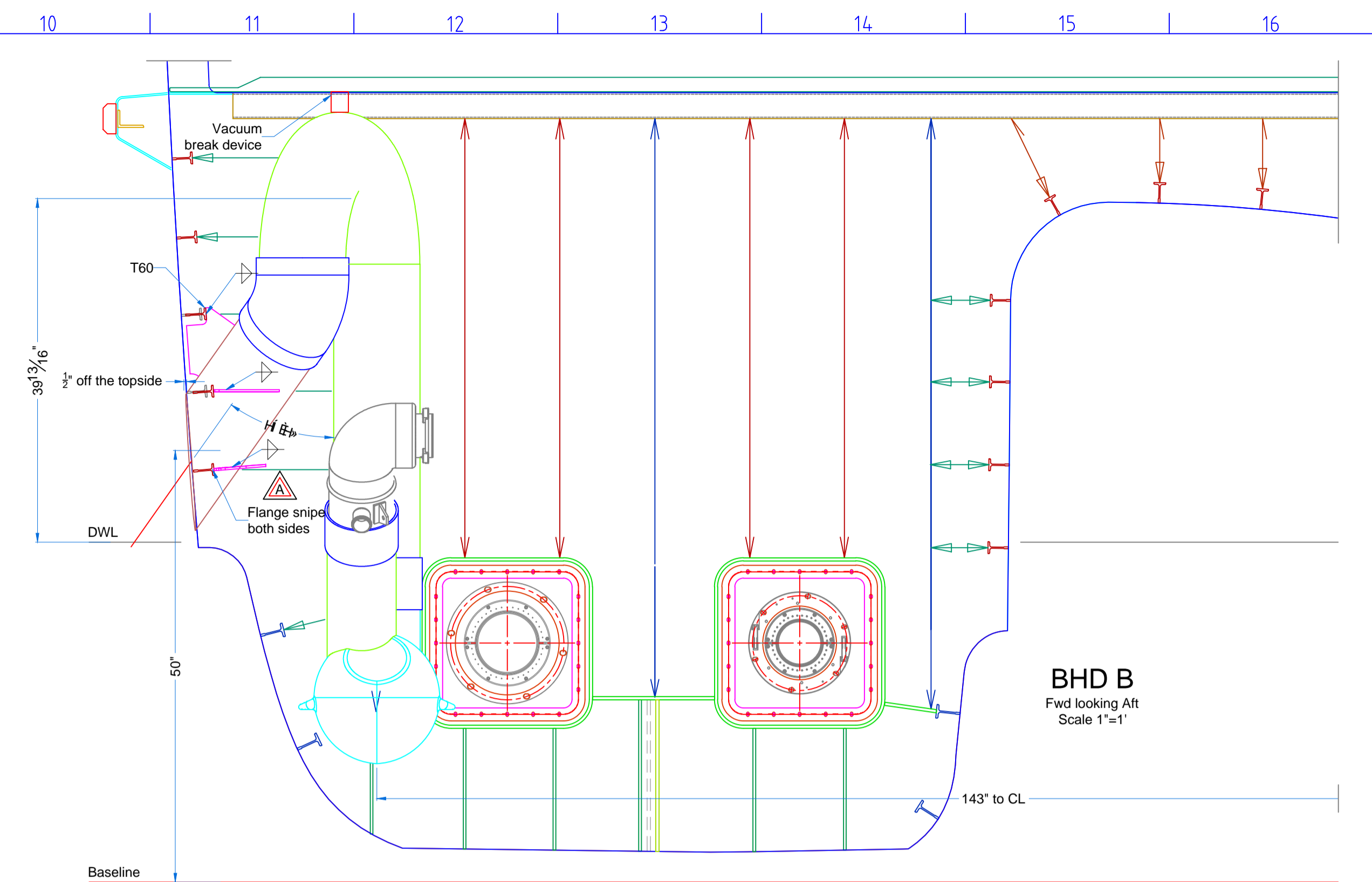
BHD B Fwd looking Aft Scale 1"=1'
