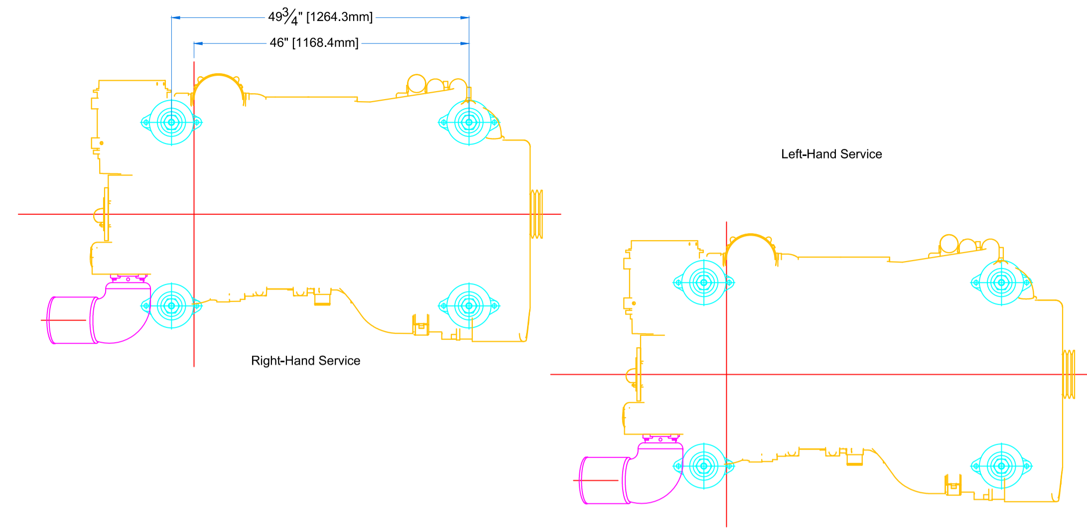
Engine Layout Schematic Scale 3/4"=1'-0"
