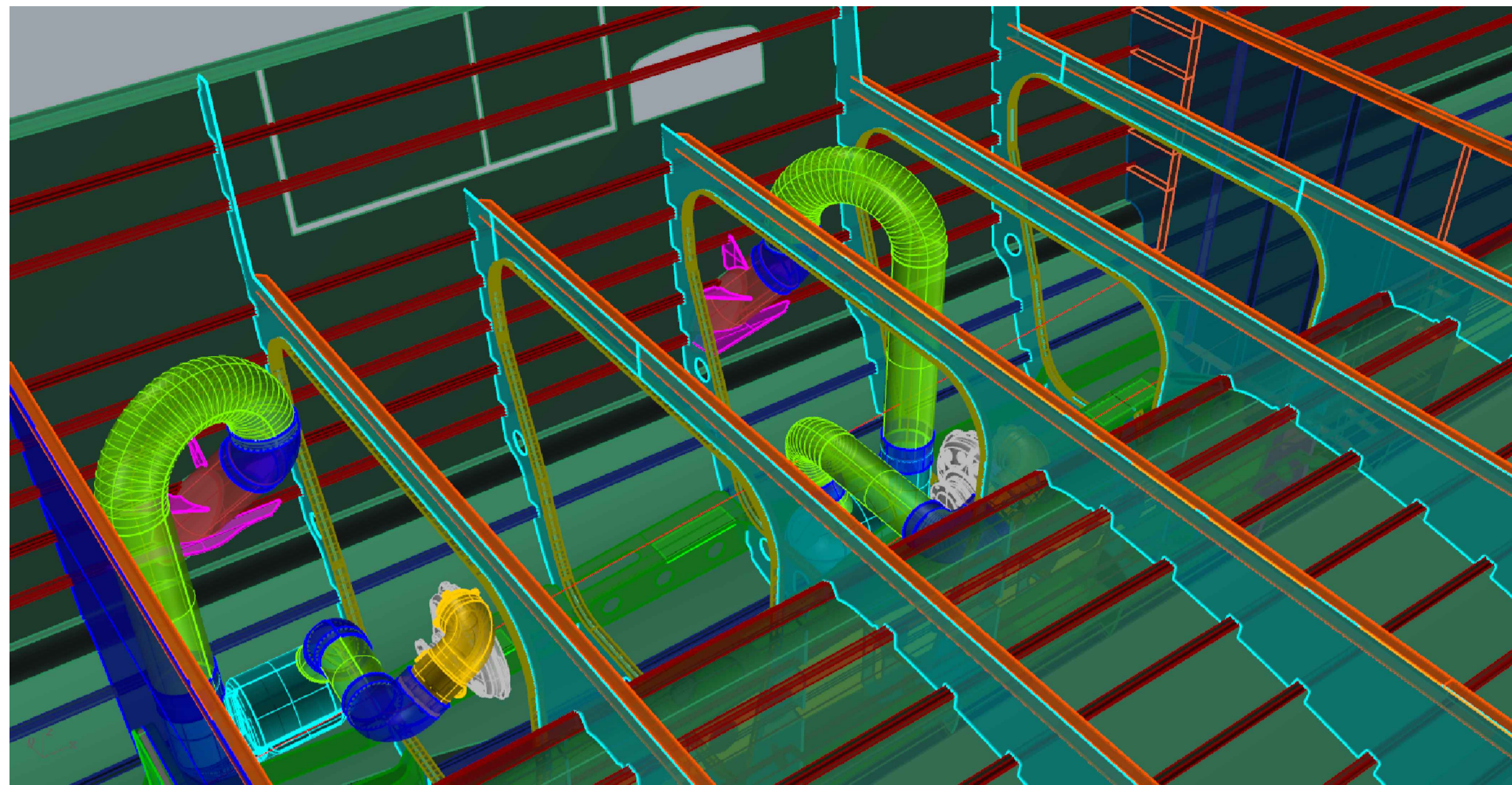
Perspective View - Port Side Looking Fwd
