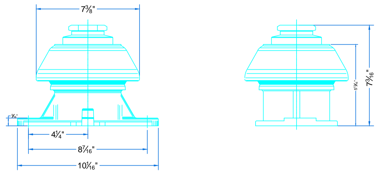
Engine Mount Detail Scale 3"=1'-0"
