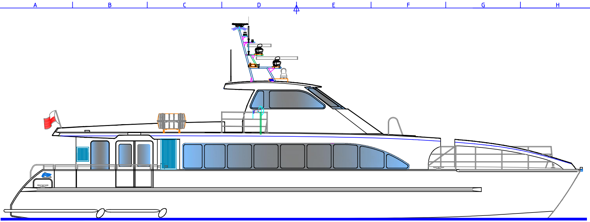
Outboard Profile
