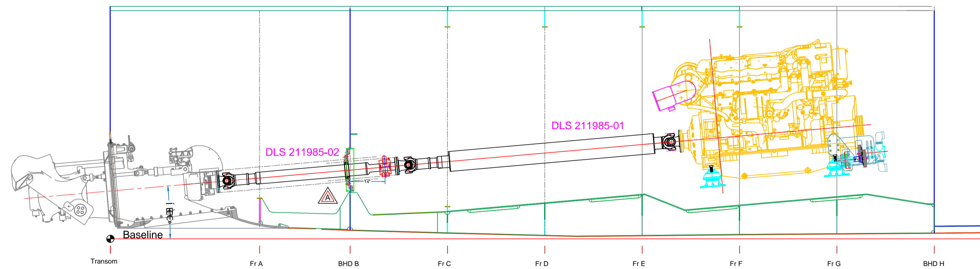
PROFILE-LONG SHAFT LINE
