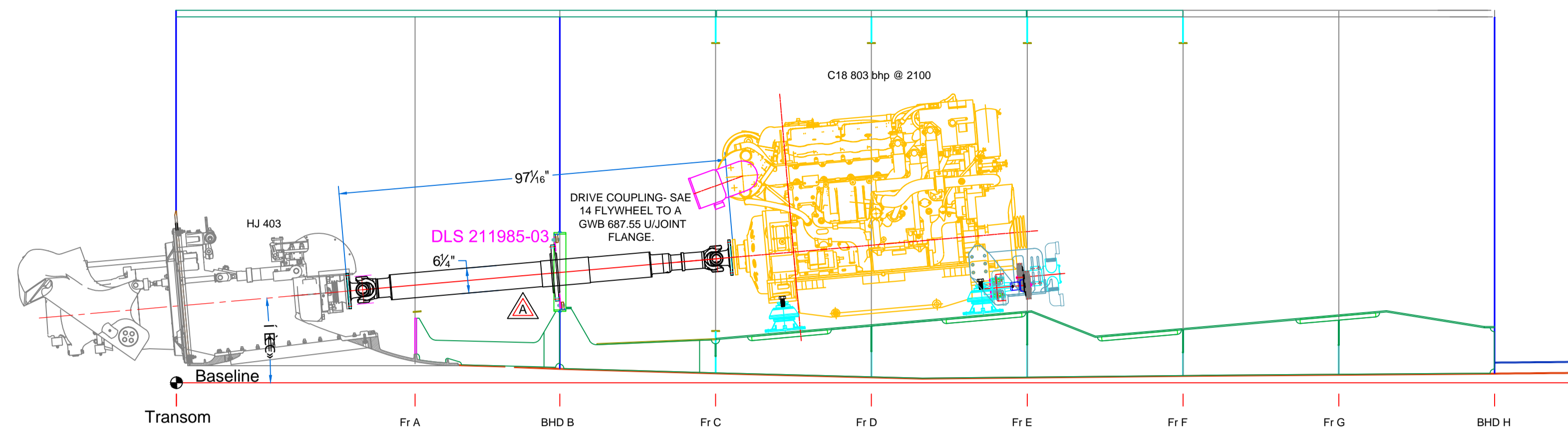
PROFILE-SHORT SHAFT LINE
