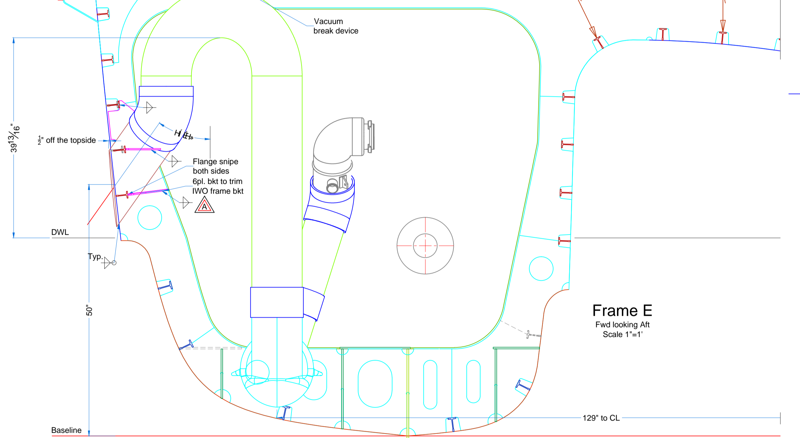
Frame E Fwd looking Aft Scale 1"=1'
