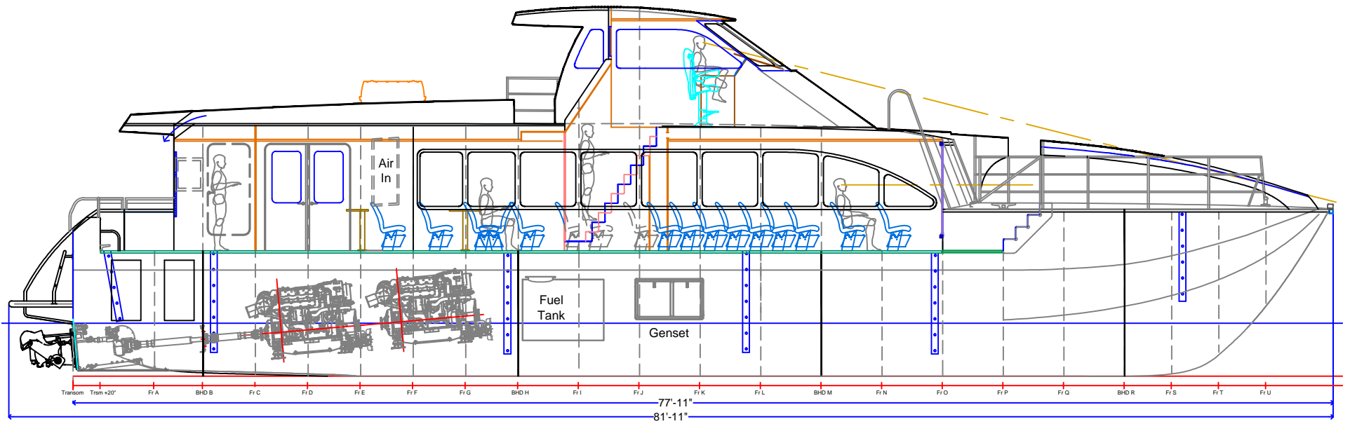
Inboard Profile
